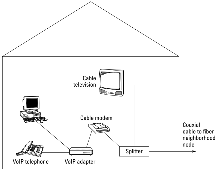
Figure 6-1: Connecting VoIP through a cable modem.
